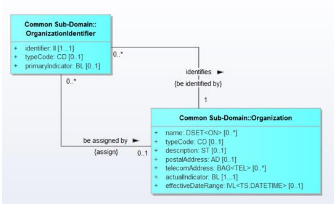
Figure 1: Example of how identifier attributes were modeled in previous releases (using a separate identifier class).
