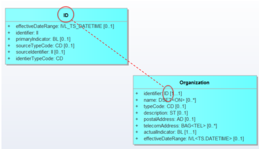
Figure 2: Example of how identifier attributes are modeled starting in BRIDG R5 (using the ID datatype class).
