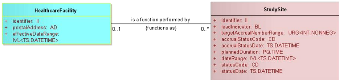
Figure A4: Example of an association between two classes
